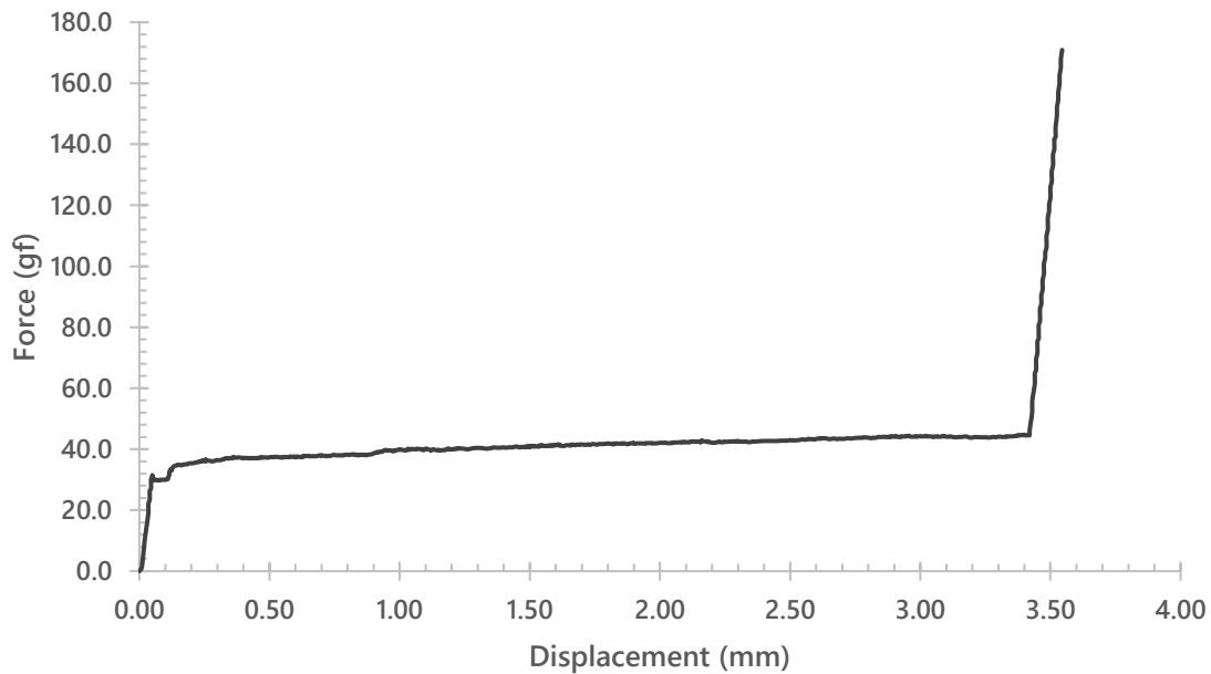
Gateron Magnetic Jade Delta Light (Upstroke)
